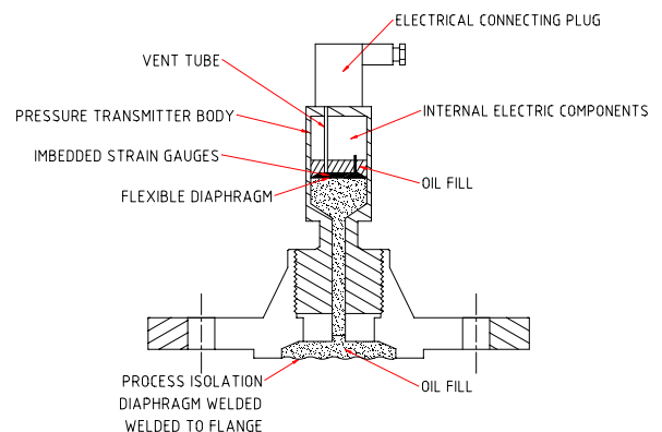
Figure 1 A style of pressure transmitter on a process seal.
